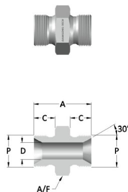
Male Adapter (BSP (Parallel) Thread)
