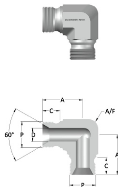
Male Union Elbow (BSP (Parallel) Thread)
