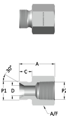
Male to Female Hose Adapter (BSP (Parallel) to BSP (Taper) Thread)
