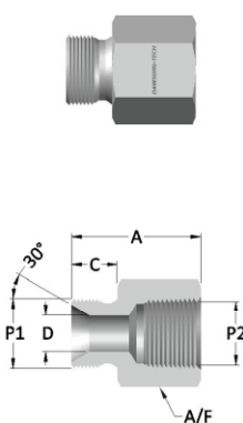
Male to Female Hose Adapter (BSP (Parallel) to NPT Thread)
