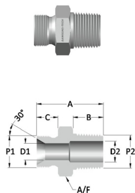
Male Adapter (BSP (Parallel) to BSP (Taper) Thread)
