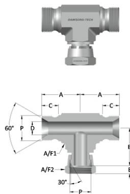
Male to Swivel Female Branch Tee (BSP (Parallel) Thread)
