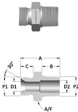
Male Adapter (BSP (Parallel) to NPT Thread)
