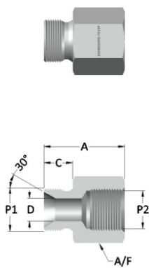
Male to Female Hose Adapter (BSP (Parallel) Thread)
