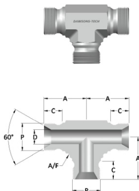
Male Union Tee (BSP (Parallel) Thread)
