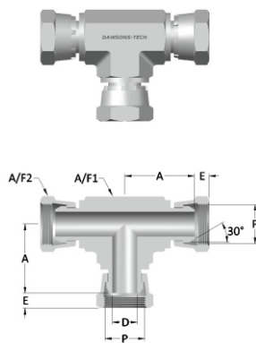
Female Swivel Union Tee (BSP (Parallel) Thread)
