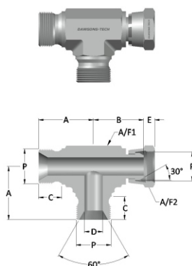
Male to Swivel Female Run Tee (BSP (Parallel) Thread)
