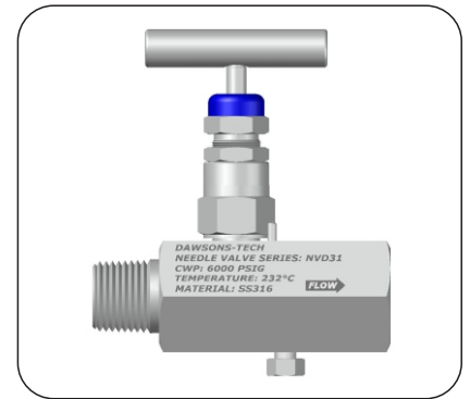
Bleeder Screw Gauge Valve Series : NVD31
