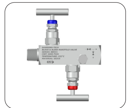
Block & Bleed Gauge Valve Series : BBGV1
